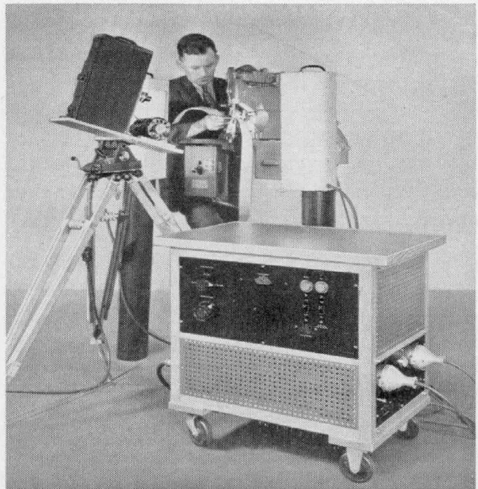
FIGURE 1. TYPE 621-H Stroboscope and TYPE 651-A Camera set up to photograph a machine for stitching leather
