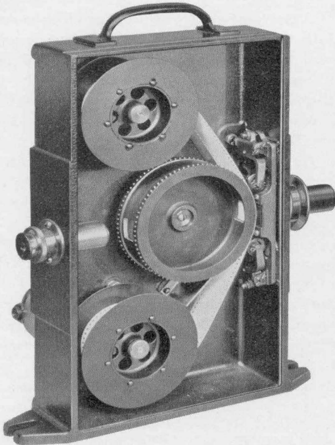
FIGURE 4. Interior view of TYPE 651-A Camera showing the film reels and sprocket
