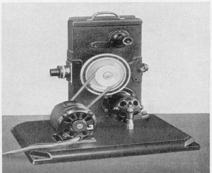
FIGURE 3. External view of TYPE 651-A Camera showing the commutator and drive motors
