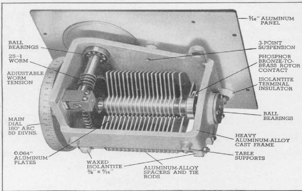
FIGURE 1. View of TYPE 722-H Precision Condenser with cabinet removed showing constructional details
