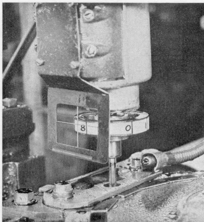
FIGURE 5. Photograph of the automatic tapping machine from which the data of Figure 6 was obtained. The drum, numbered in sections, and the cross hairs were attached in order that the pictures might be accurately analyzed. This arrangement makes it possible to measure the angular displacement accurately for each frame of the motion picture film
