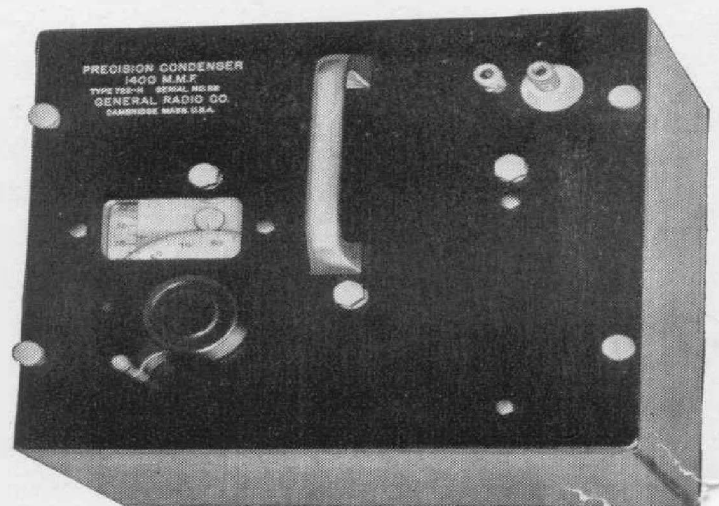
FIGURE 2. Panel view of TYPE 722-H Precision Condenser
